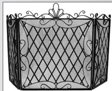
FS1 Large Fire Screen with wings Overall ht 920mm Height of panels 770mm Width of main panel 760mm Width of wings 360mm
